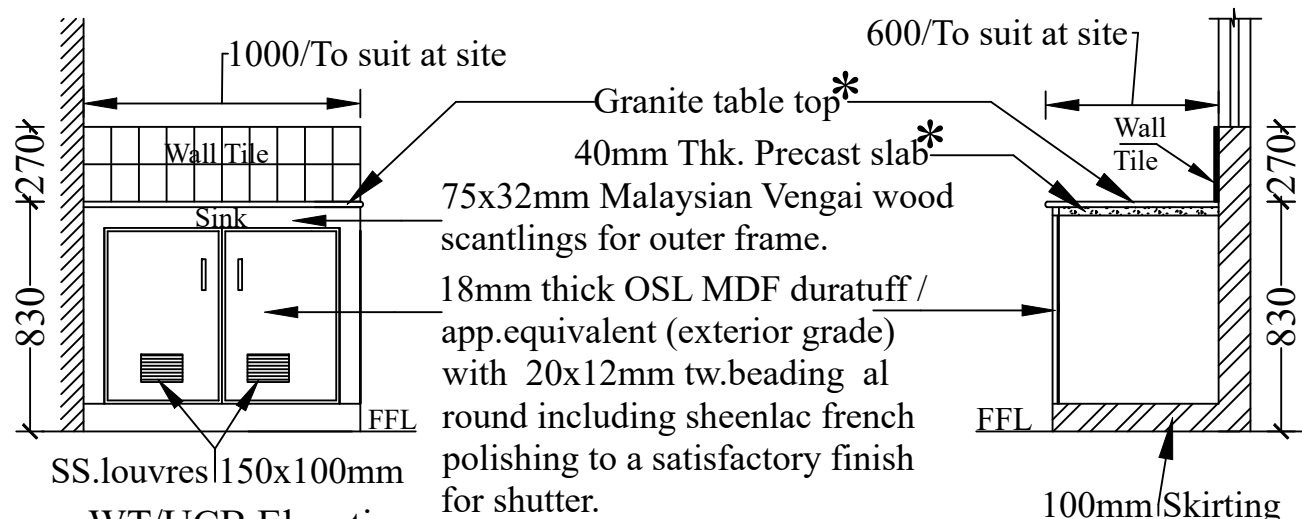
WT/UCB Elevation
