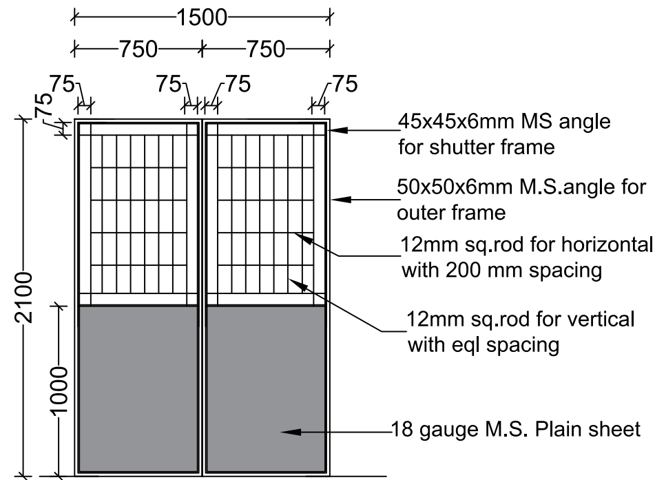
GRILL DOOR- GD SIZE : 1500X2100mm SCHEDULE ITEM NO:
