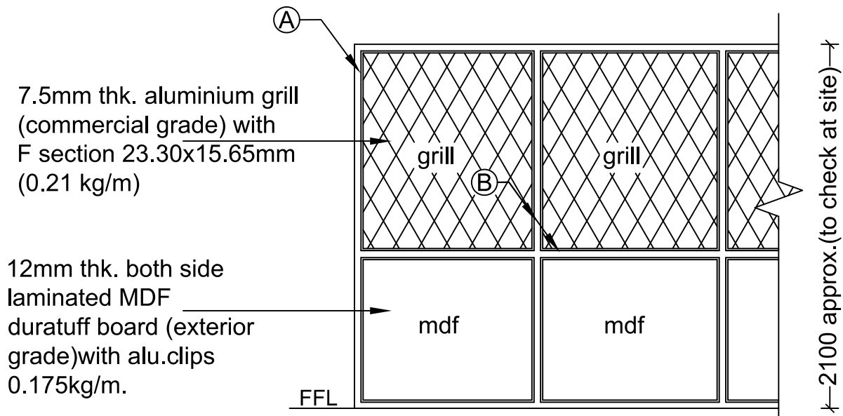
ALUMINIUM PARTITION With Grill (typical)
