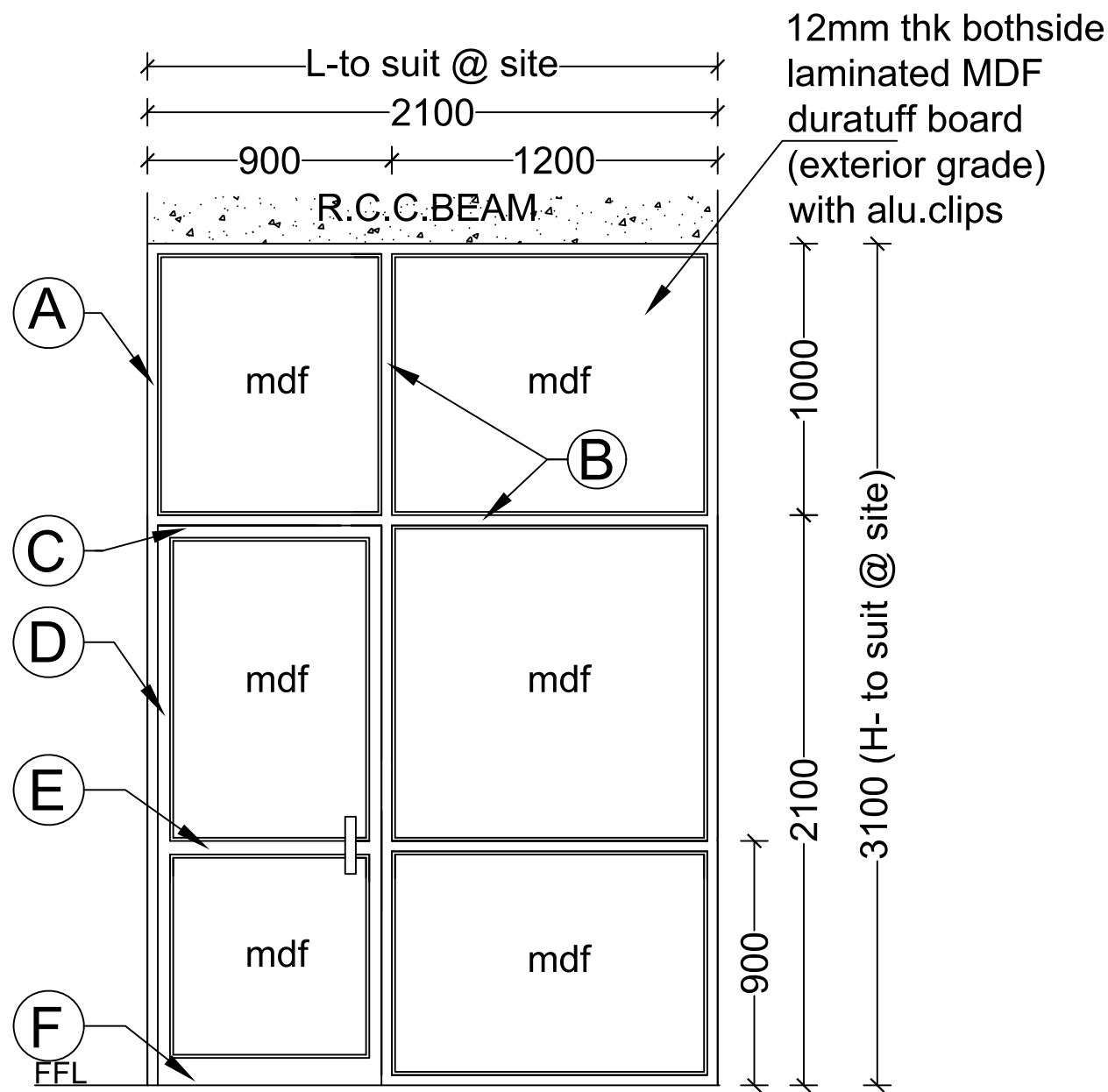
Aluminium Partition with Door: 2100x3100mm
