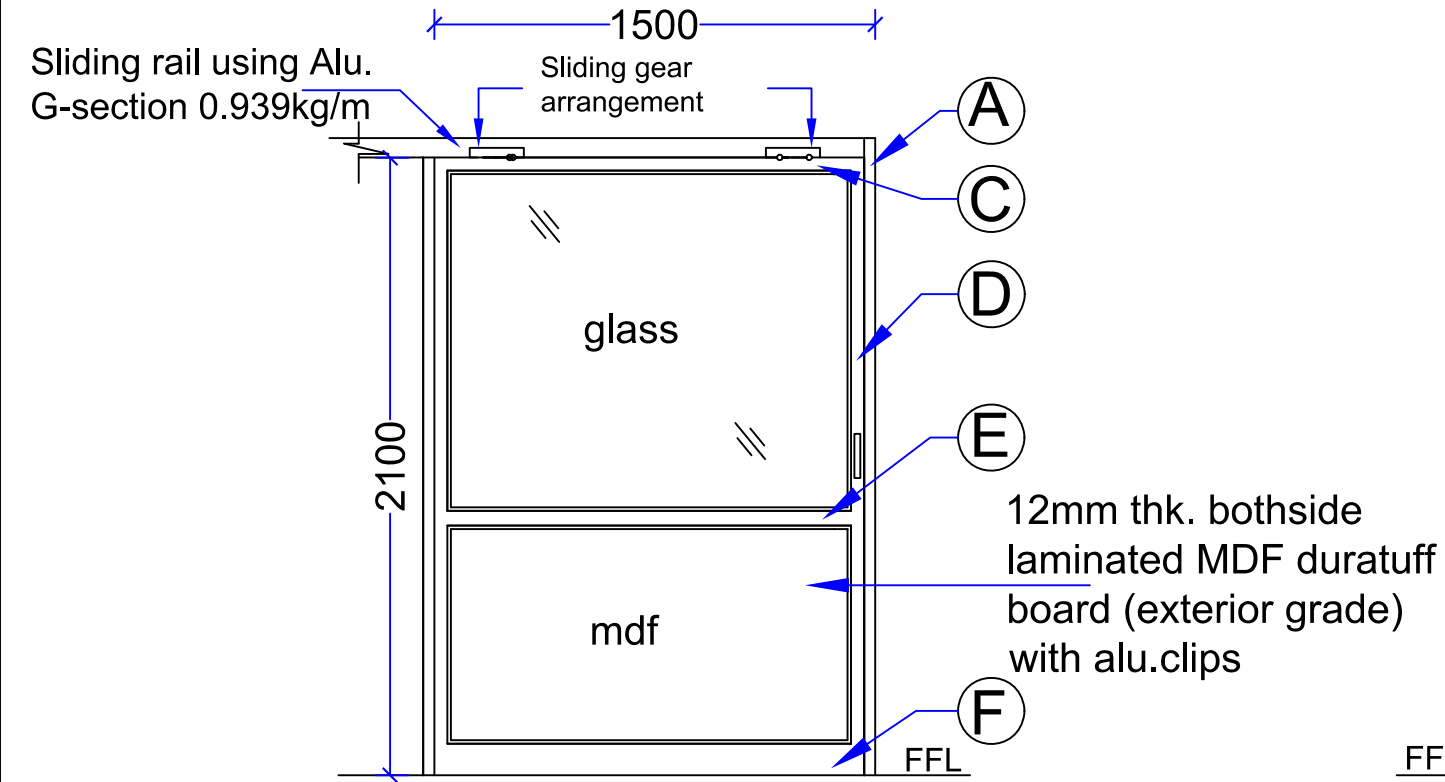
Alu. Sliding Door: 1500x2100mm-SD Schedule Item No: 50(b)
