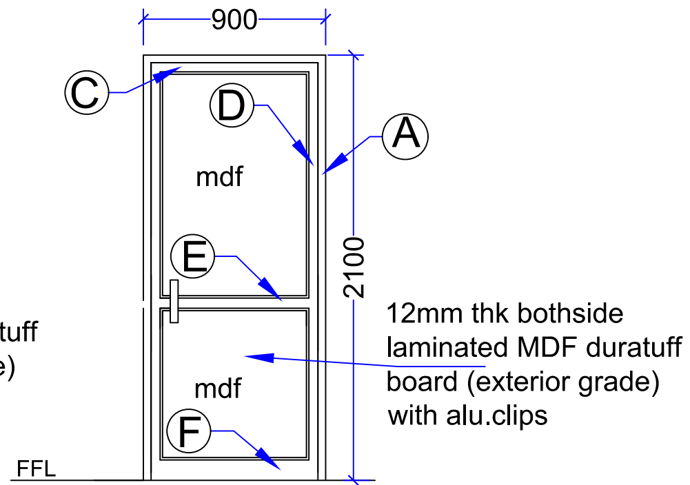
(Door Size:900x2100mm - AD1) Schedule Item No: 50(a)
