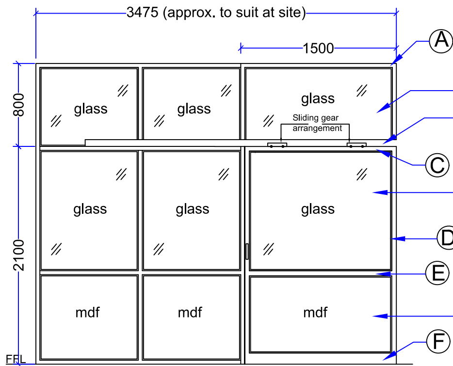
ALUMINIUM PARTITION WITH SLIDING DOOR - 1575x2380mm (VIEW-4) SD1 - 1500x2100mm Schedule Item No: 50(c)
