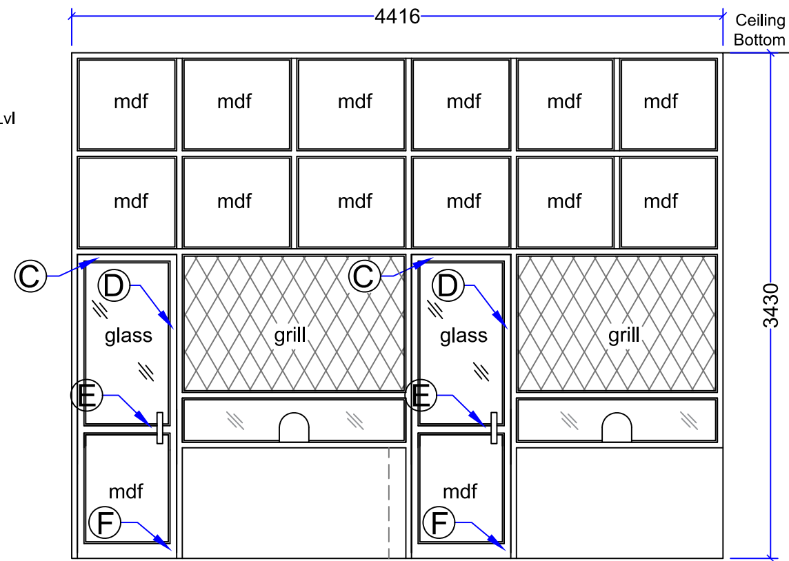
ALUMINIUM PARTITION - 4415x3430mm (View-6) (Door Size: 750x2100mm - AD2) Schedule Item No: Sch-B-20(a)
