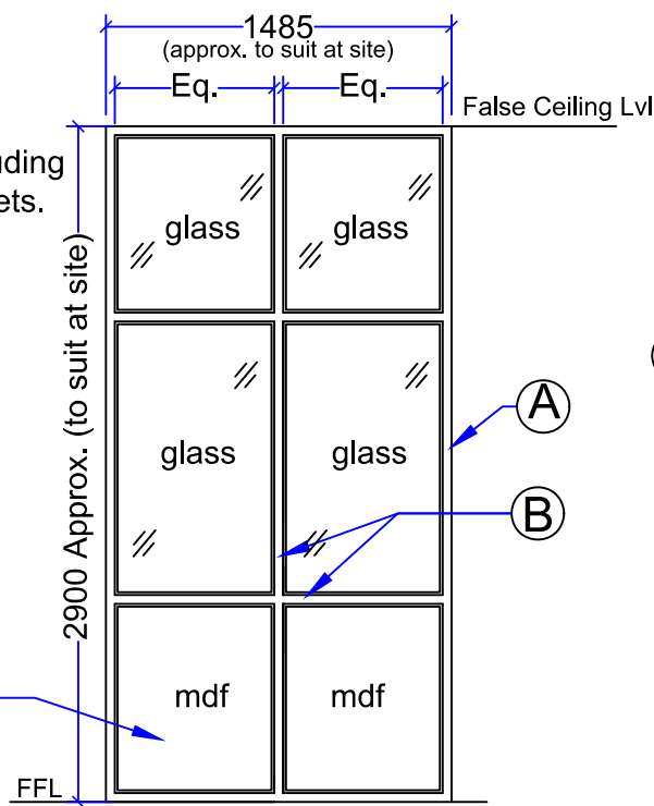
ALUMINIUM PARTITION - 1485x2800mm (View-5) Schedule Item No: 50(c)
