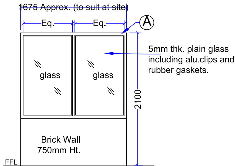
View-7 ALUMINIUM PARTITION WITH DOOR Size: 1675x1350mm (Approx.) Schedule Item No: Sch-B 20(b)
