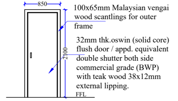
Leadlined Door - LD Size: 850 x 2100mm Schedule Item no: 37a
