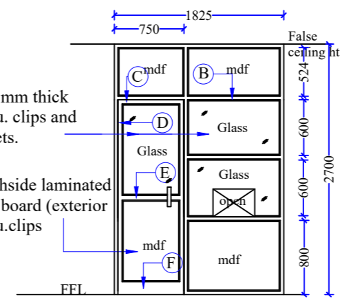
VIEW - 3 Aluminium partition with door @ Dose admin area Size: 1825x2700mm Door Size: D2- 750x2100mm Schedule item No: 38c
