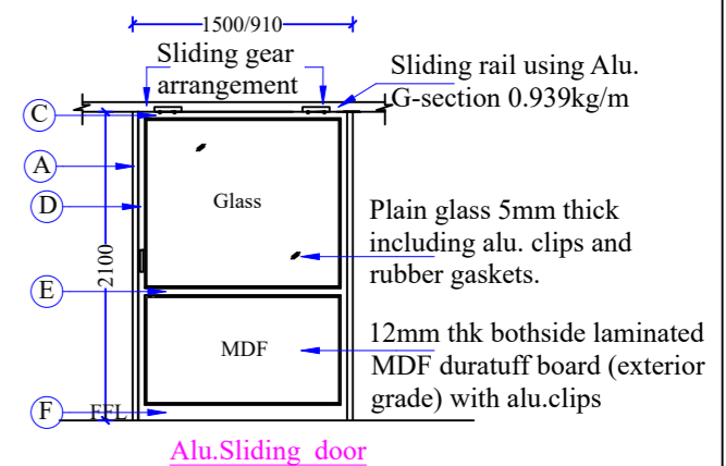
Alu. Sliding door Sd - 1500 x 2100mm Schedule item no: 40a Sd1 - 910 x 2100mm Schedule item no: 40b
