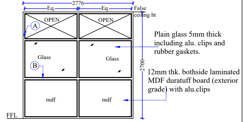
VIEW - 4 Aluminium partition @ Dose admin area Size: 2775x2700mm Schedule item No: 38b
