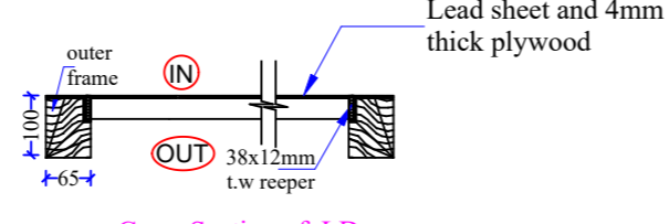
Cross Section of LD
