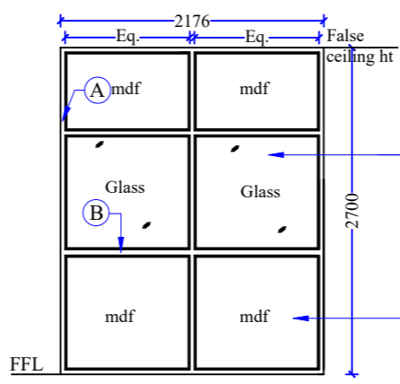
VIEW - 2 Aluminium partition @ clean room Size: 2175x2700mm Schedule item No: 38d
