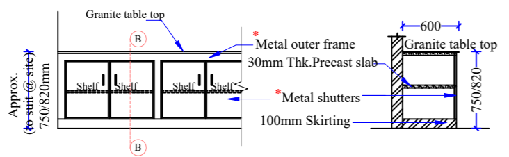
WT / UCB @ waste store room (TYPICAL) Schedule item no: 41a
