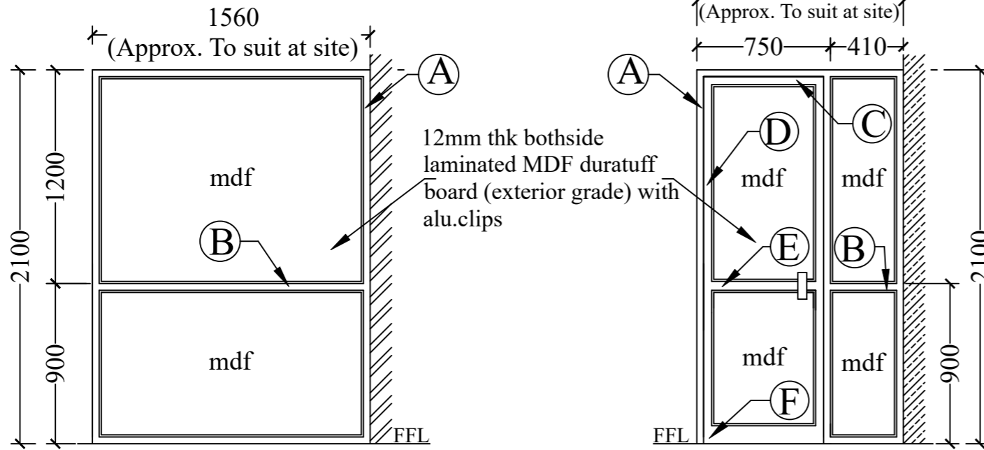
ALUMINIUM PARTITION SIZE -1560x2100mm Schedule Item No: 47(b)
