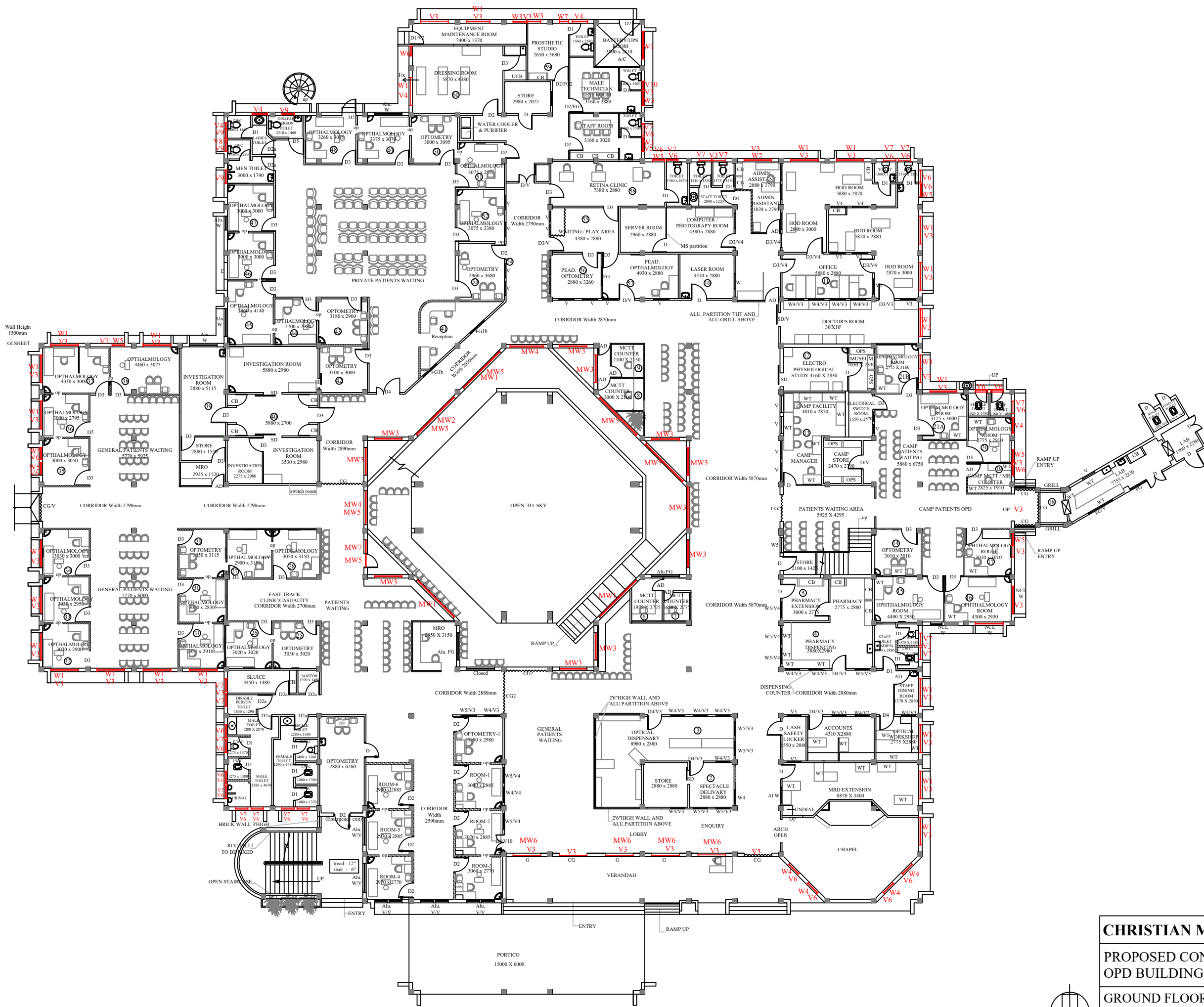
GROUND FLOOR PLAN 2713.25SQM /29194.57SQFT
