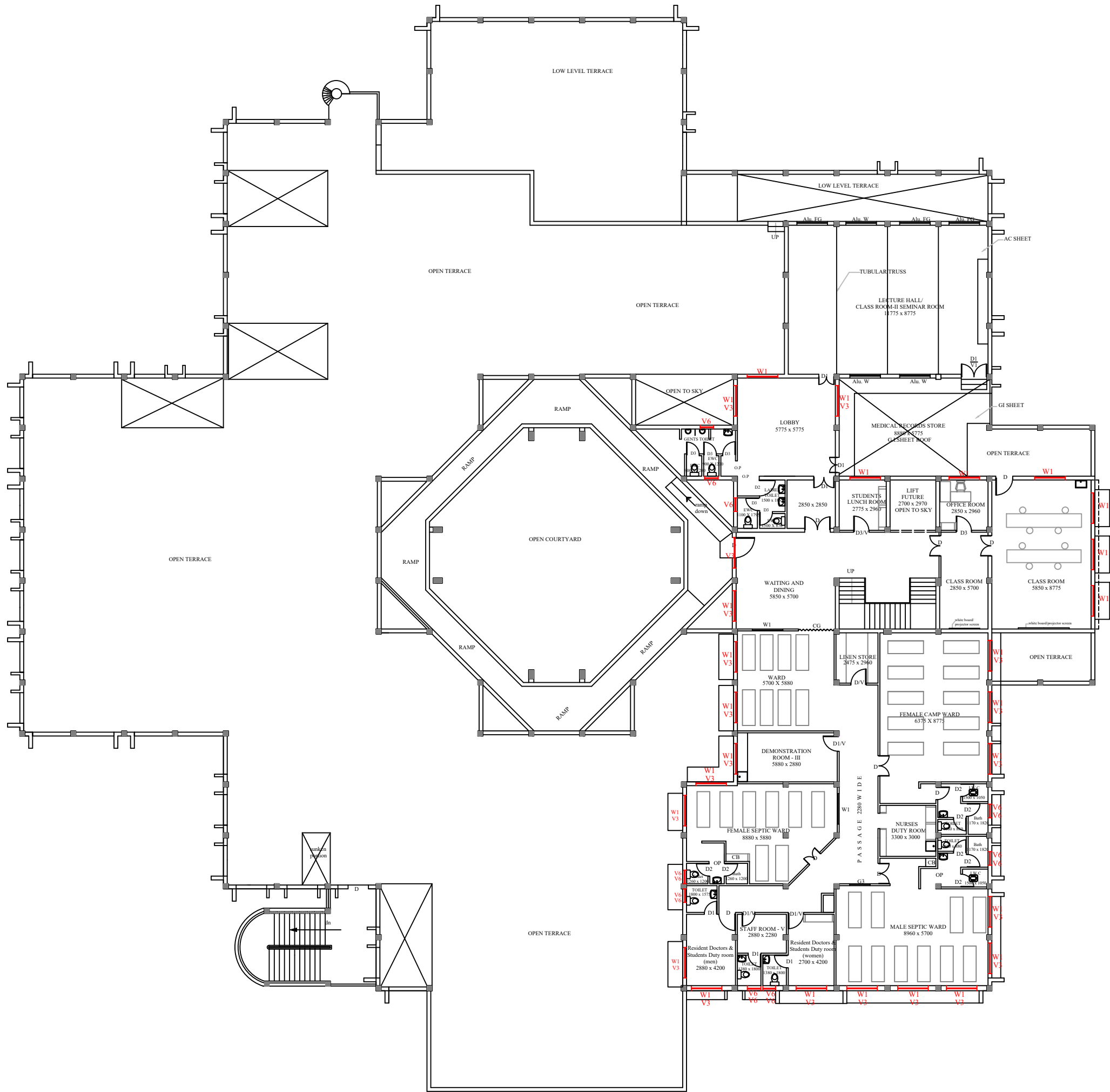
SECOND FLOOR PLAN 760.90SQM / 8187.28SQFT
